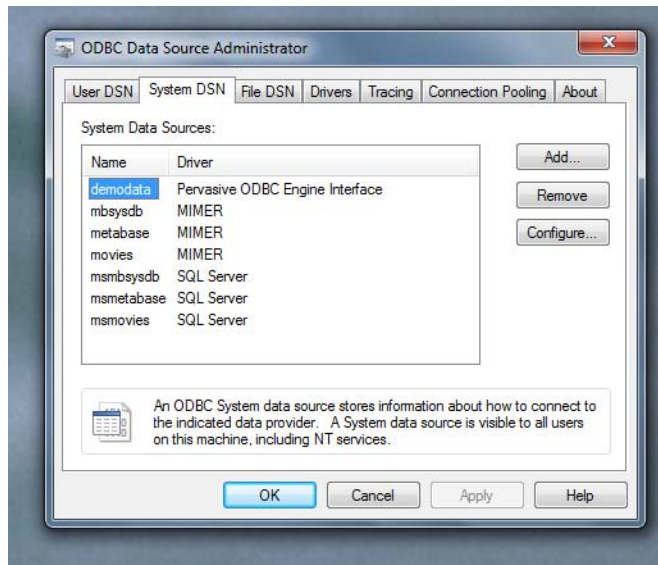
Figure 7. MS SQL ODBC connection screen to Metabase databases.
