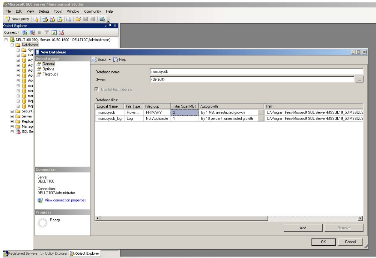
Figure 9. Defining a new MS SQL Database with SQL Server Management Studio.
