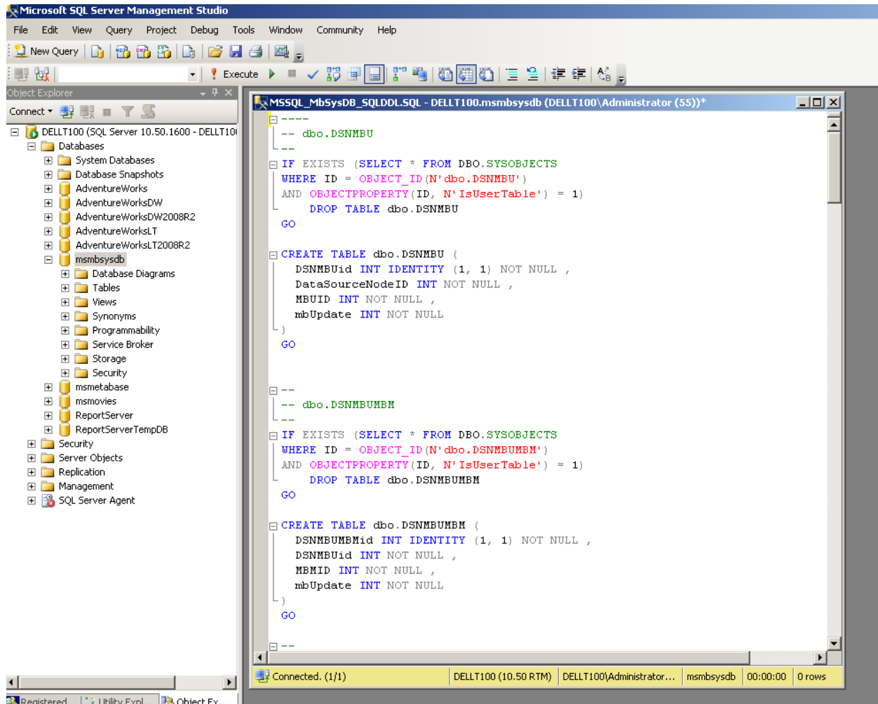
Figure 10. Defining Tables and Indexes for msmbysdb Metabase Database.
