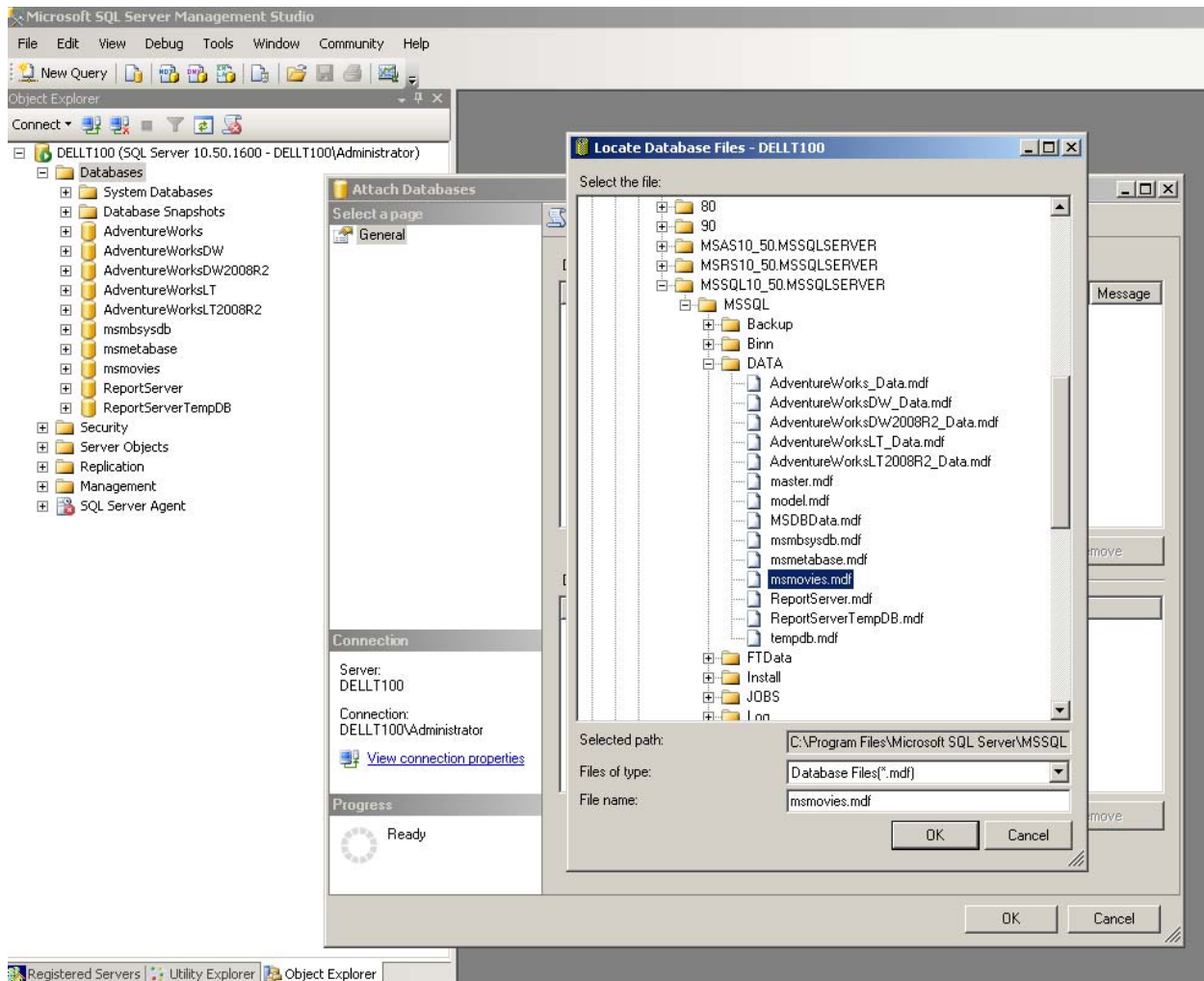
Figure 6. Attaching a Metabase Database, msmovies to MS SQL.
