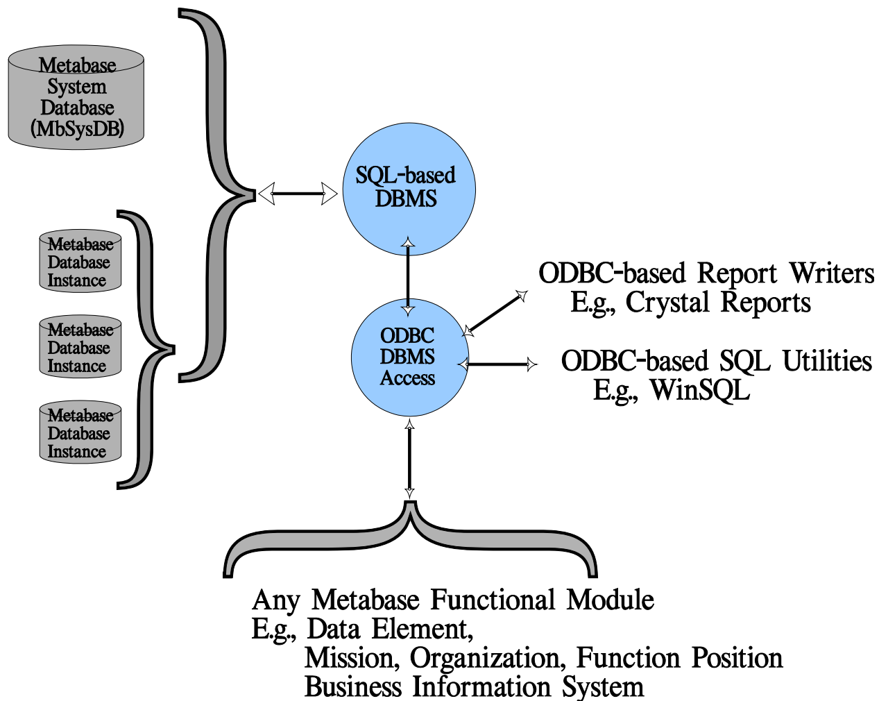
Figure 1. Metabase System Architecture.
